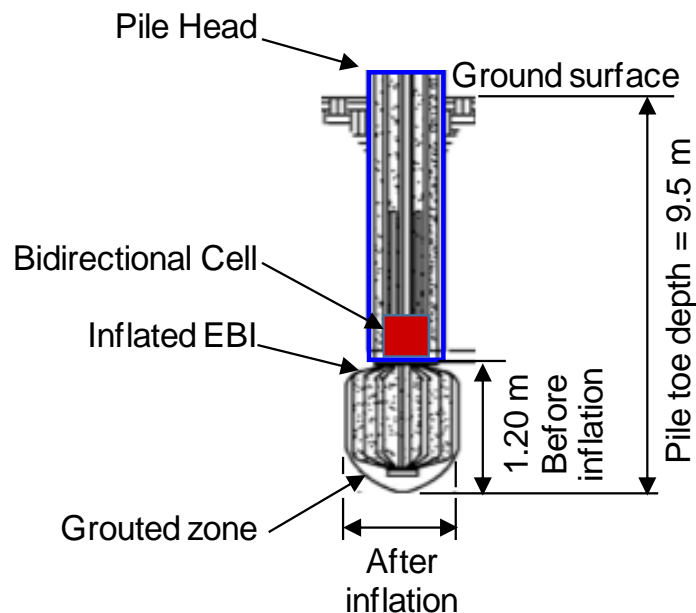
Fig. 4. Sketch showing the EB and BD arrangement (not to scale).
