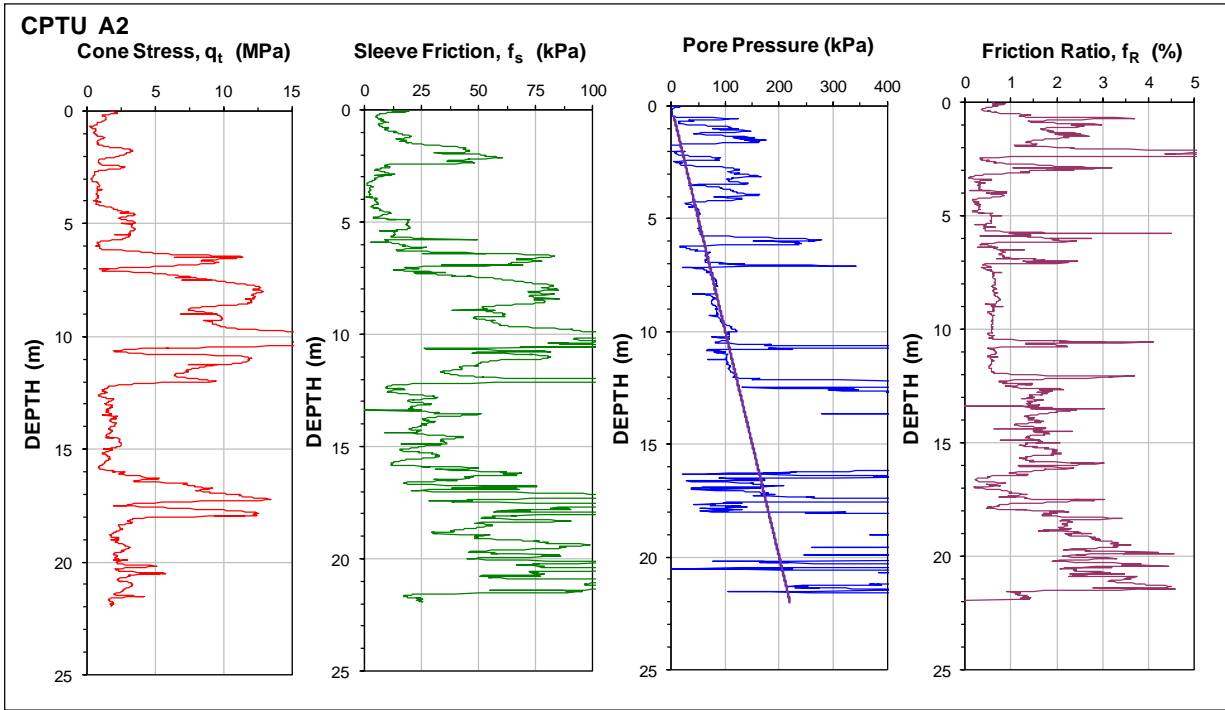
Fig. 18. Results of CPTU A2.
