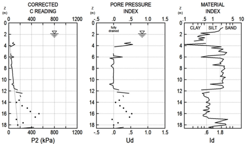
Fig. 40. DMT results, G1.
