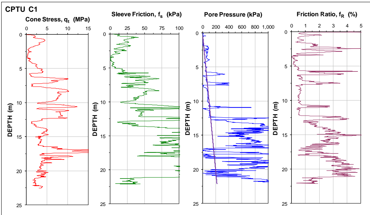
Fig. 22. Results of CPTU C1.
