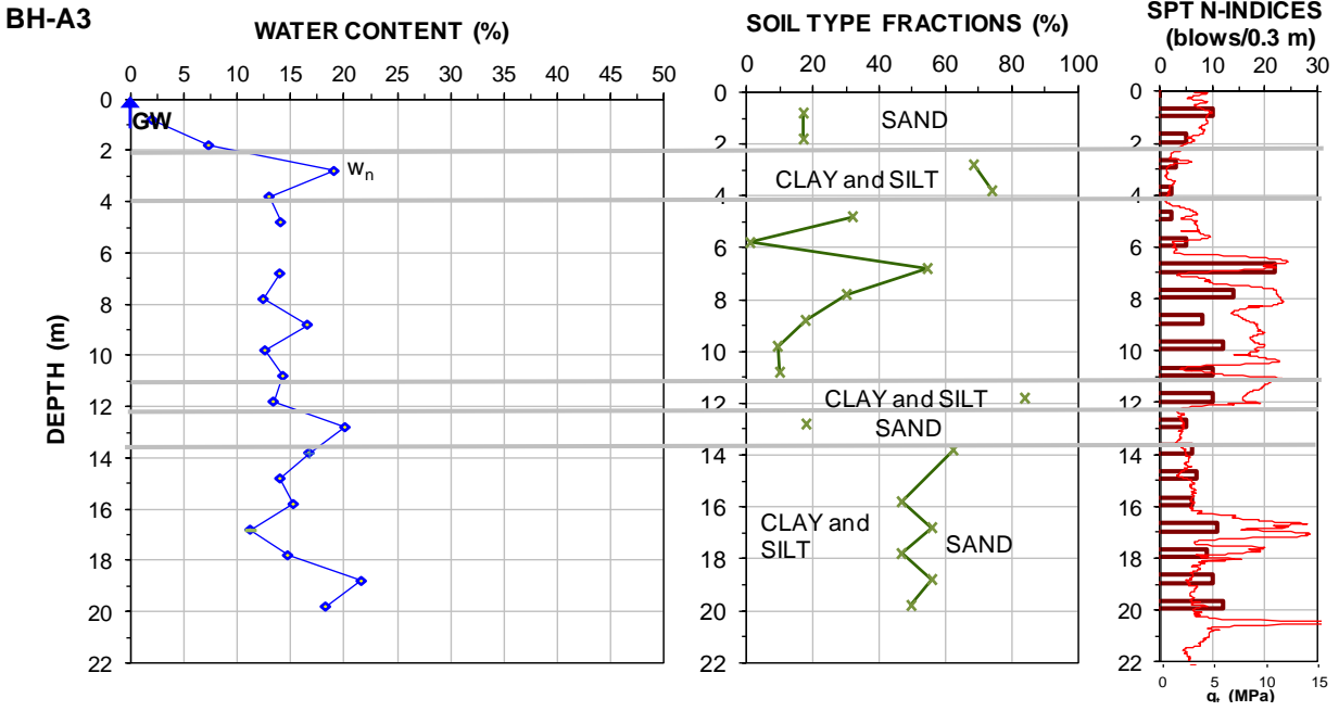
Fig. 8. Borehole data and SPT N-values, BH-A3.
