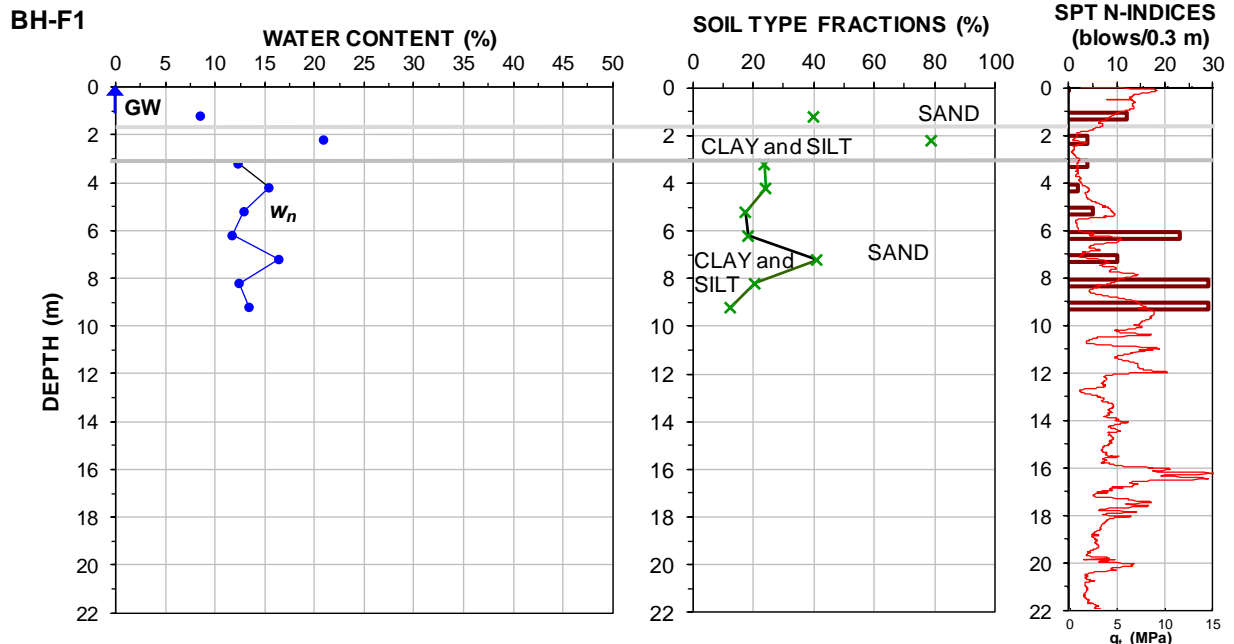
Fig. 14. Borehole data and SPT N-values, BH-F1.
