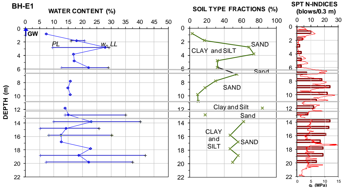
Fig. 12. Borehole data and SPT N-values, BH-E1.
