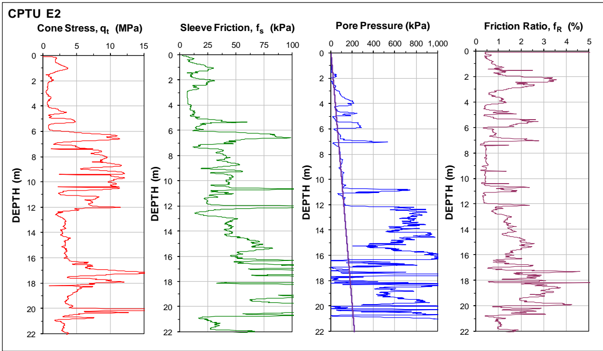
Fig. 26. Results of CPTU E2.
