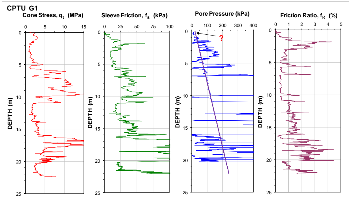
Fig. 30. Results of CPTU G1.
