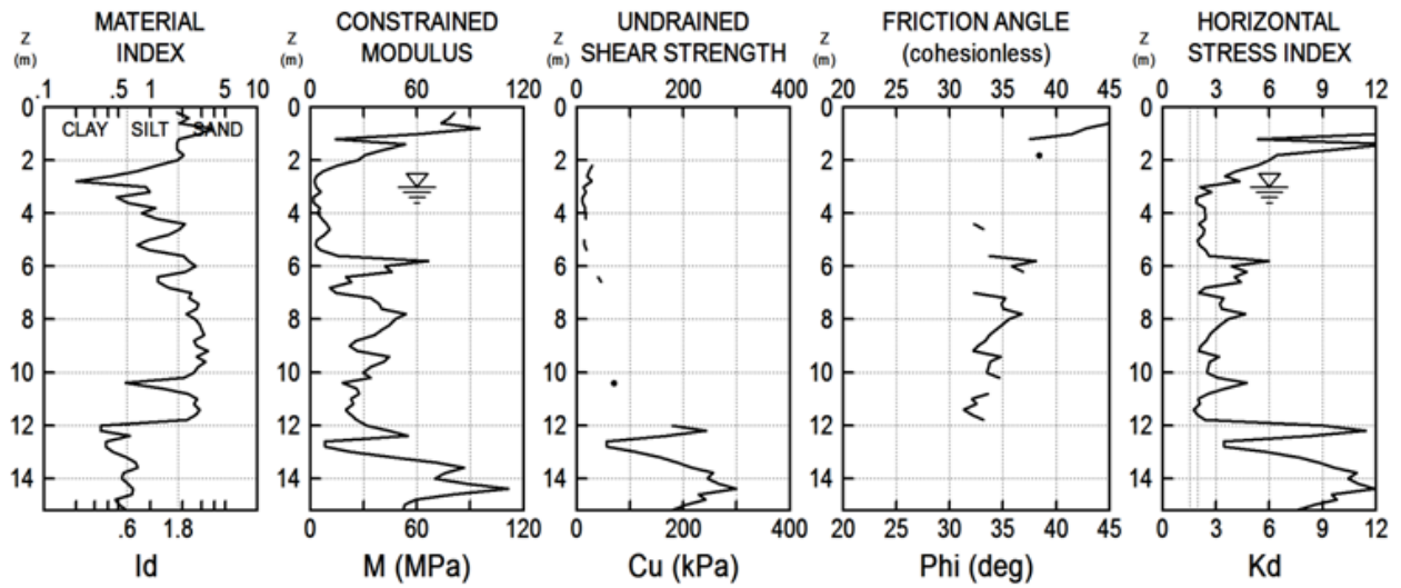
Fig. 34. DMT results, C1.
