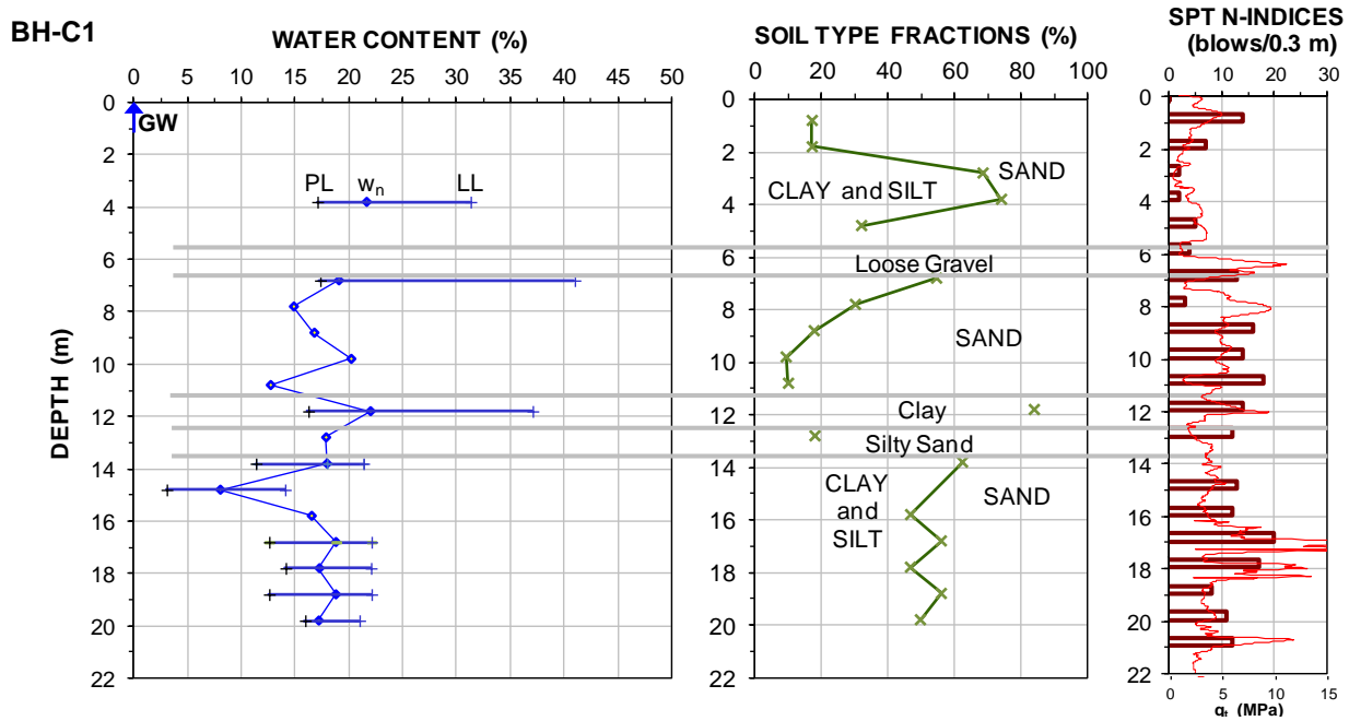
Fig. 10. Borehole data and SPT N-values, BH-C1.
