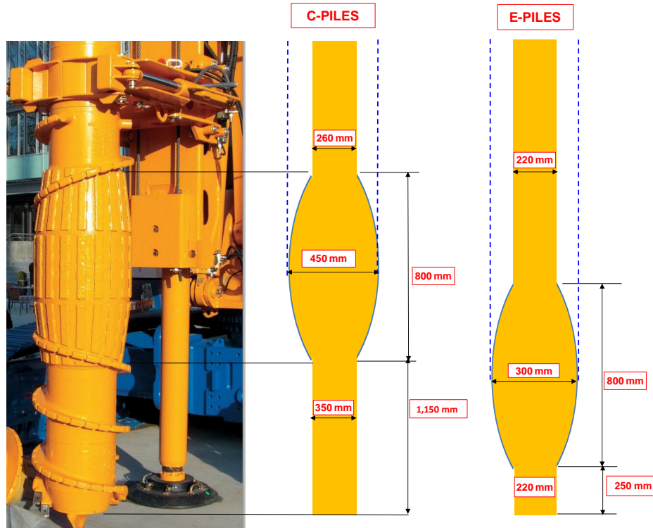
Fig. 5. Sketch showing equipment and geometry of the full displacement pile (not to scale).
