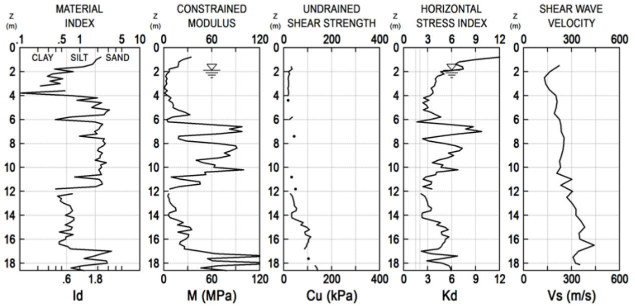
Fig. 39. DMT results, G1.
