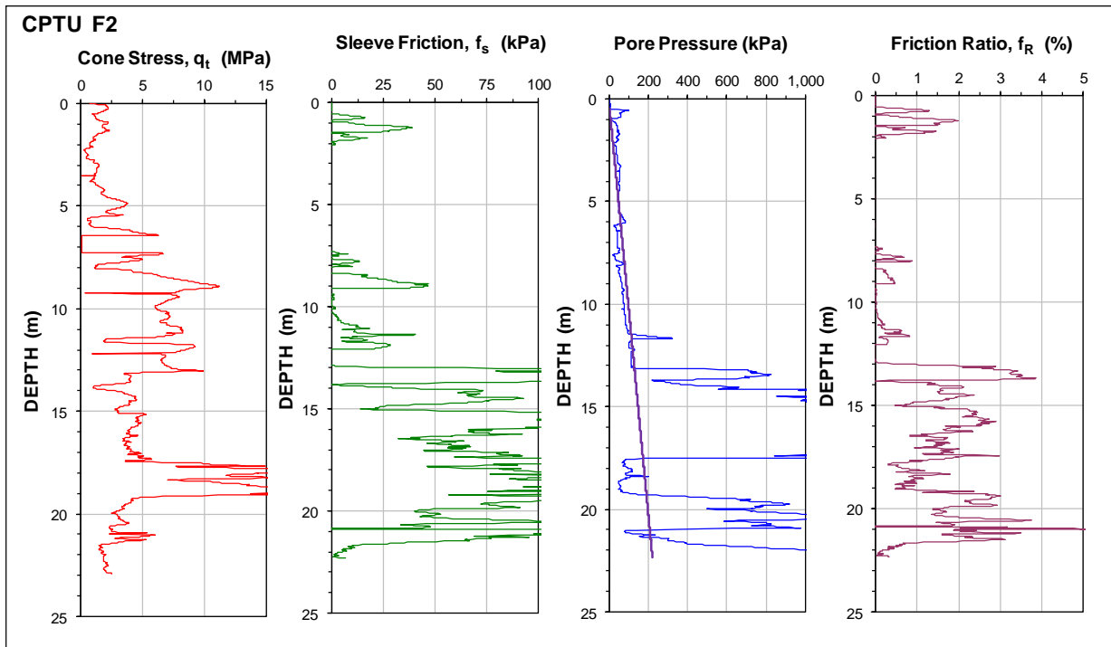
Fig. 28. Results of CPTU F2.
