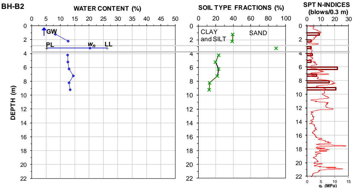
Fig. 9. Borehole data and SPT N-values, BH-B2.
