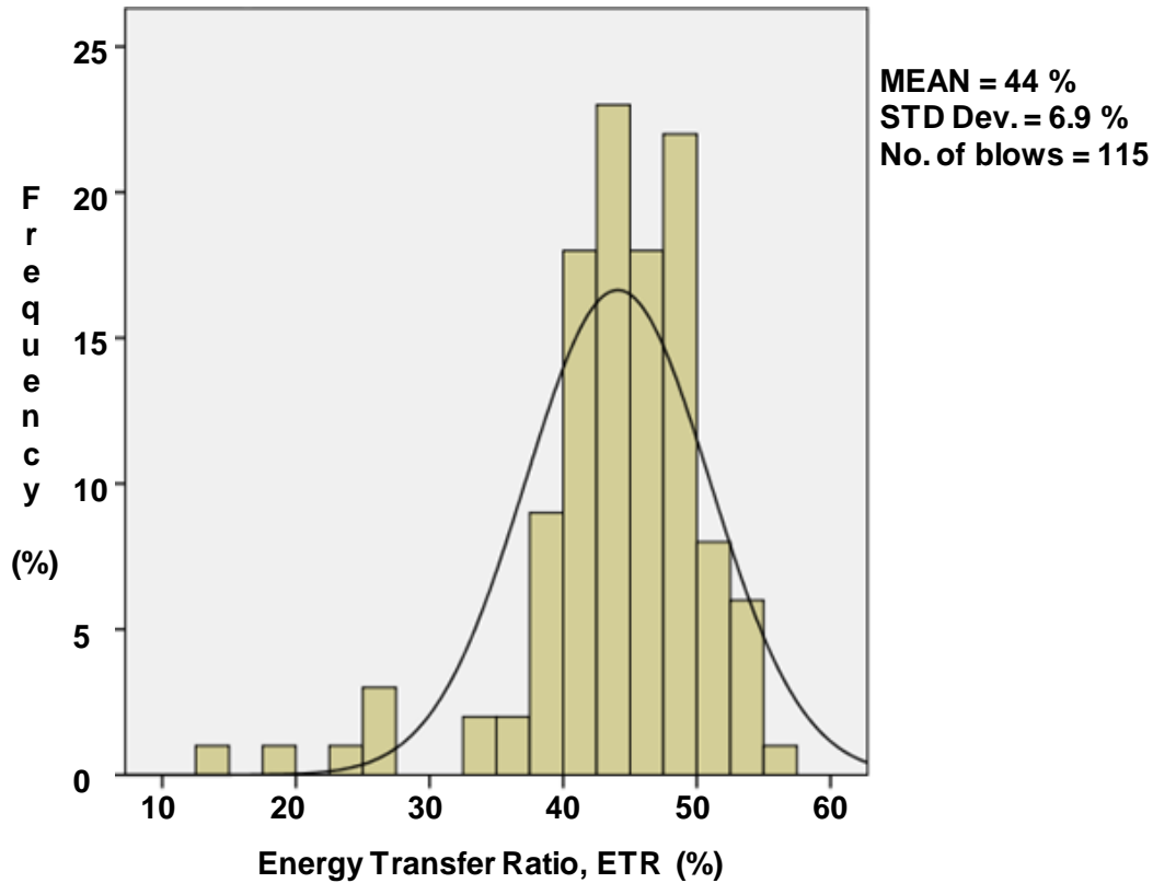
Fig. 7. Histogram of transferred energy at BH-B2, depths 6 m through 9.5 m.
