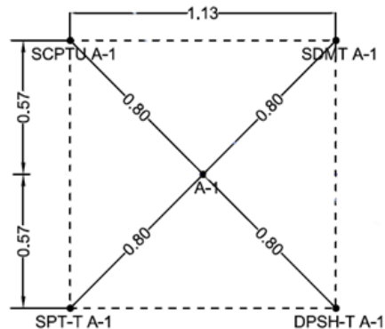
Fig. 2. Example of layout of tests performed adjacent to Pile A-1.
