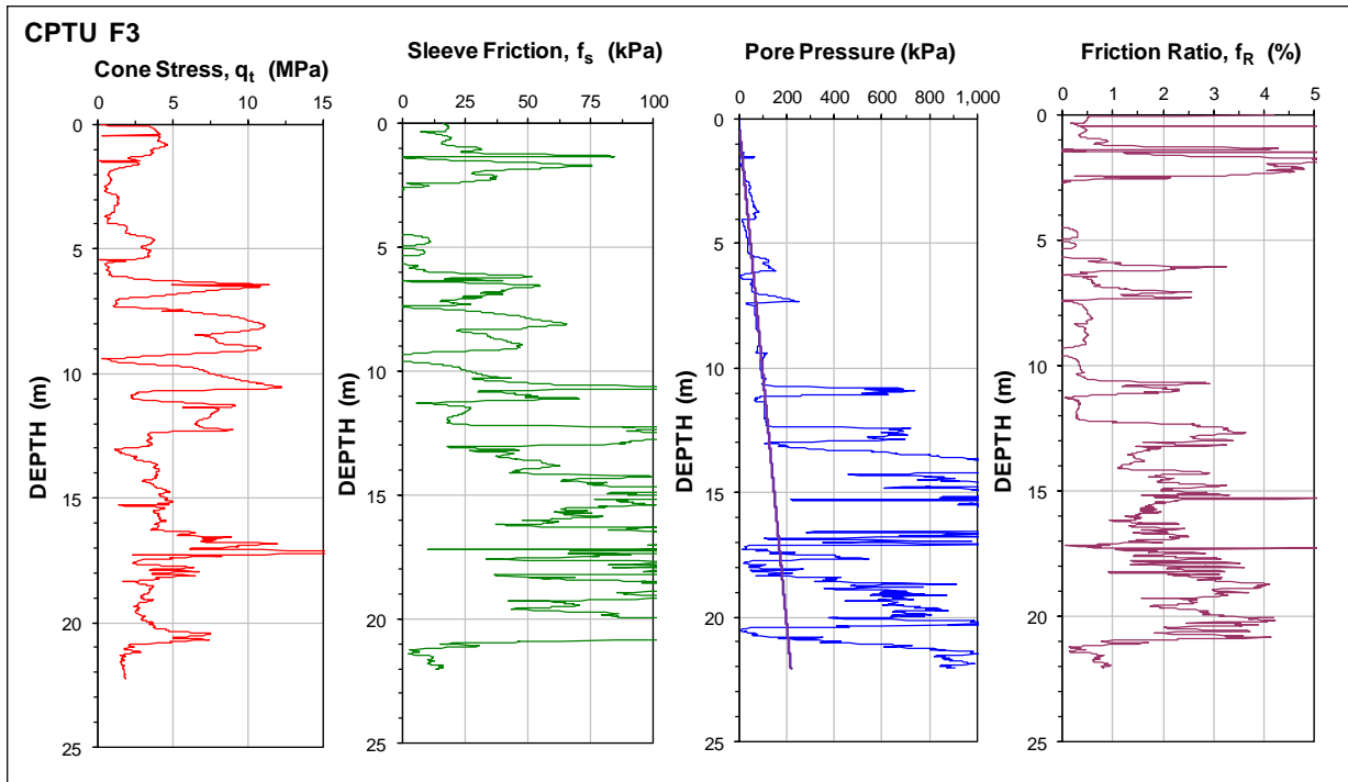
Fig. 29. Results of CPTU F3.
