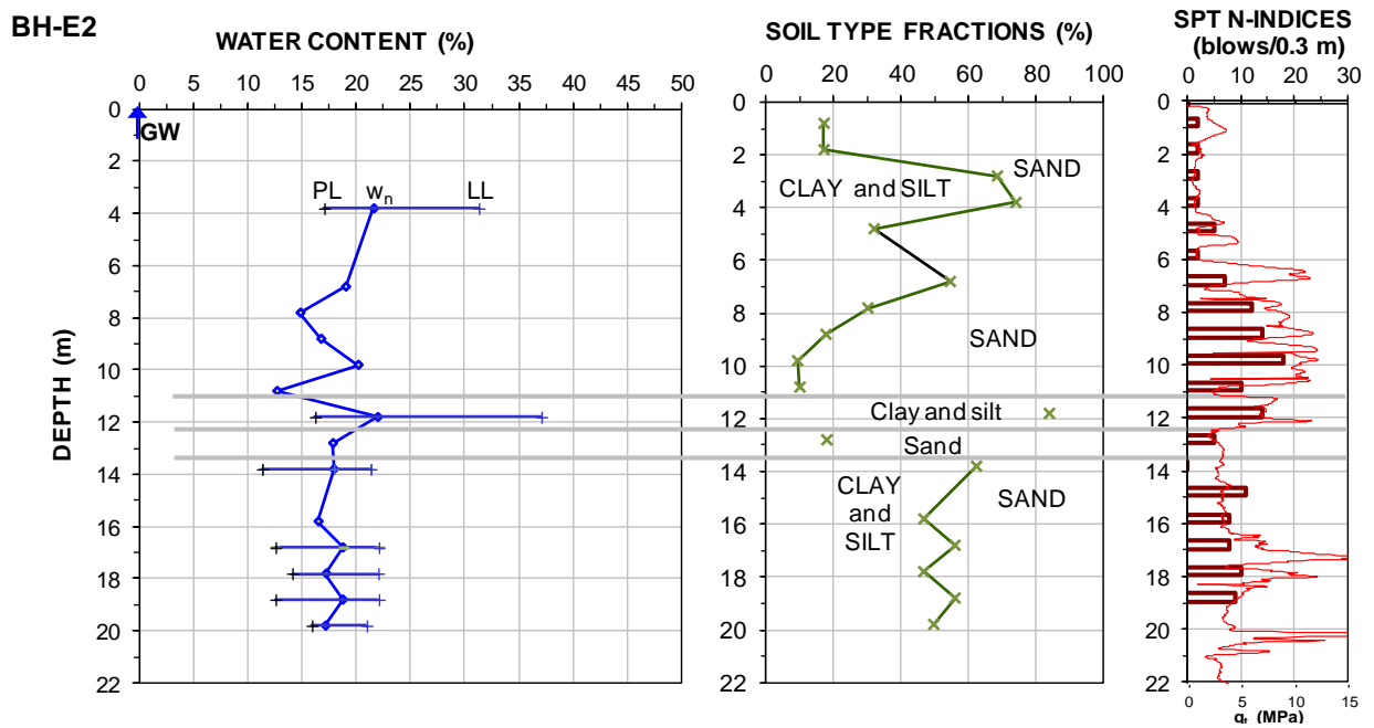
Fig. 13. Borehole data and SPT N-values, BH-E2.
