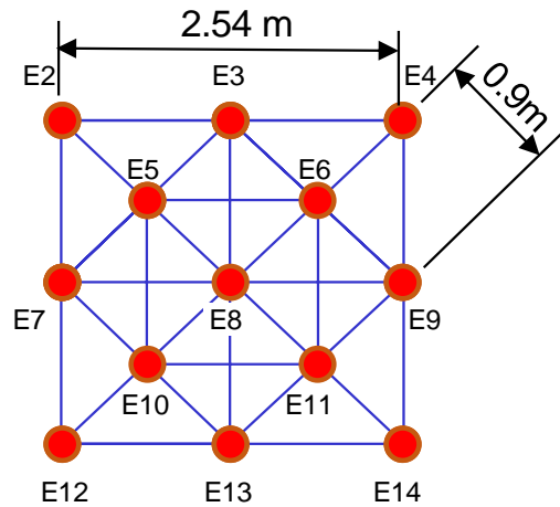
Fig. 6. B.E.S.T. Pile group configuration (E2 – E14).
