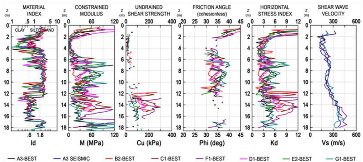
Fig. 31. Compilation of all DMT results.
