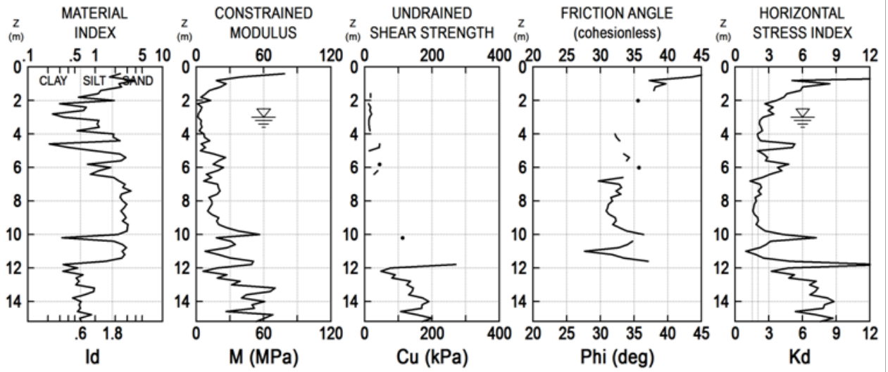
Fig. 33. DMT results, B2
