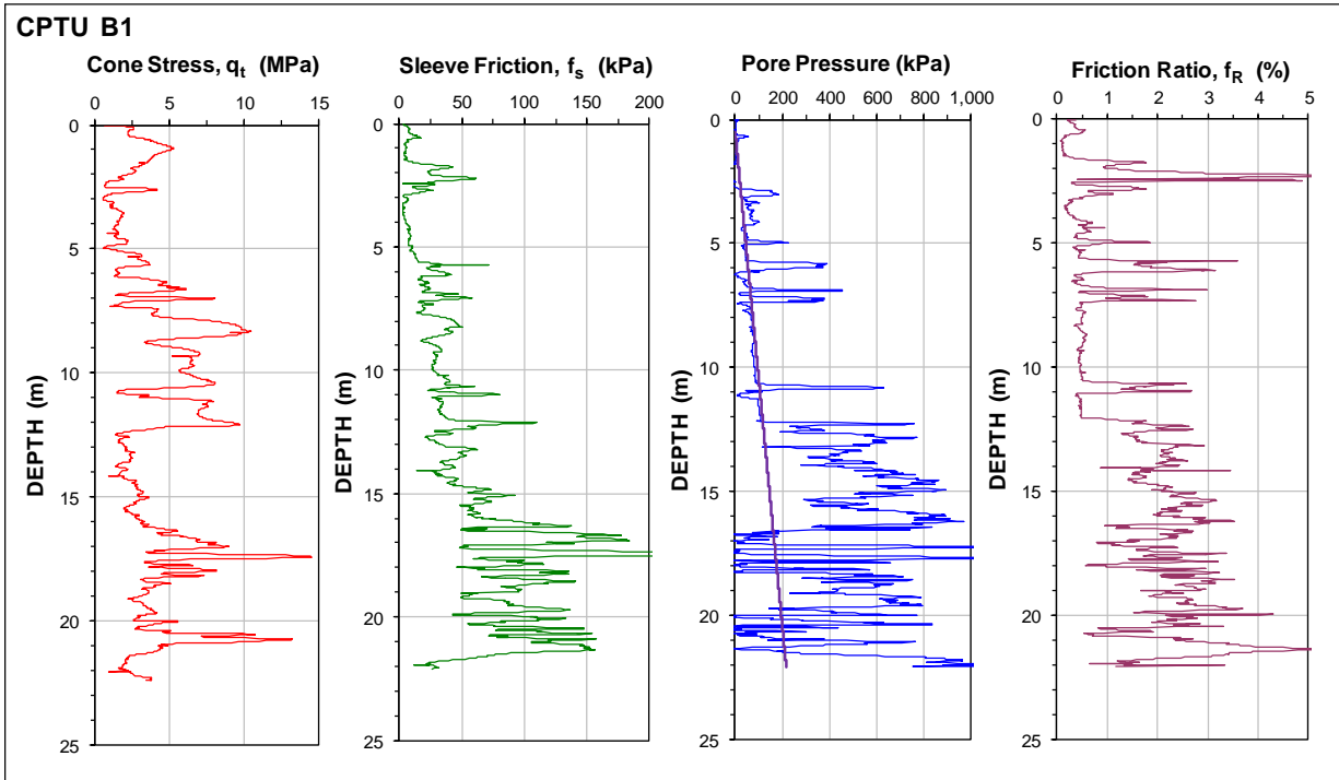
Fig. 20. Results of CPTU B1.
