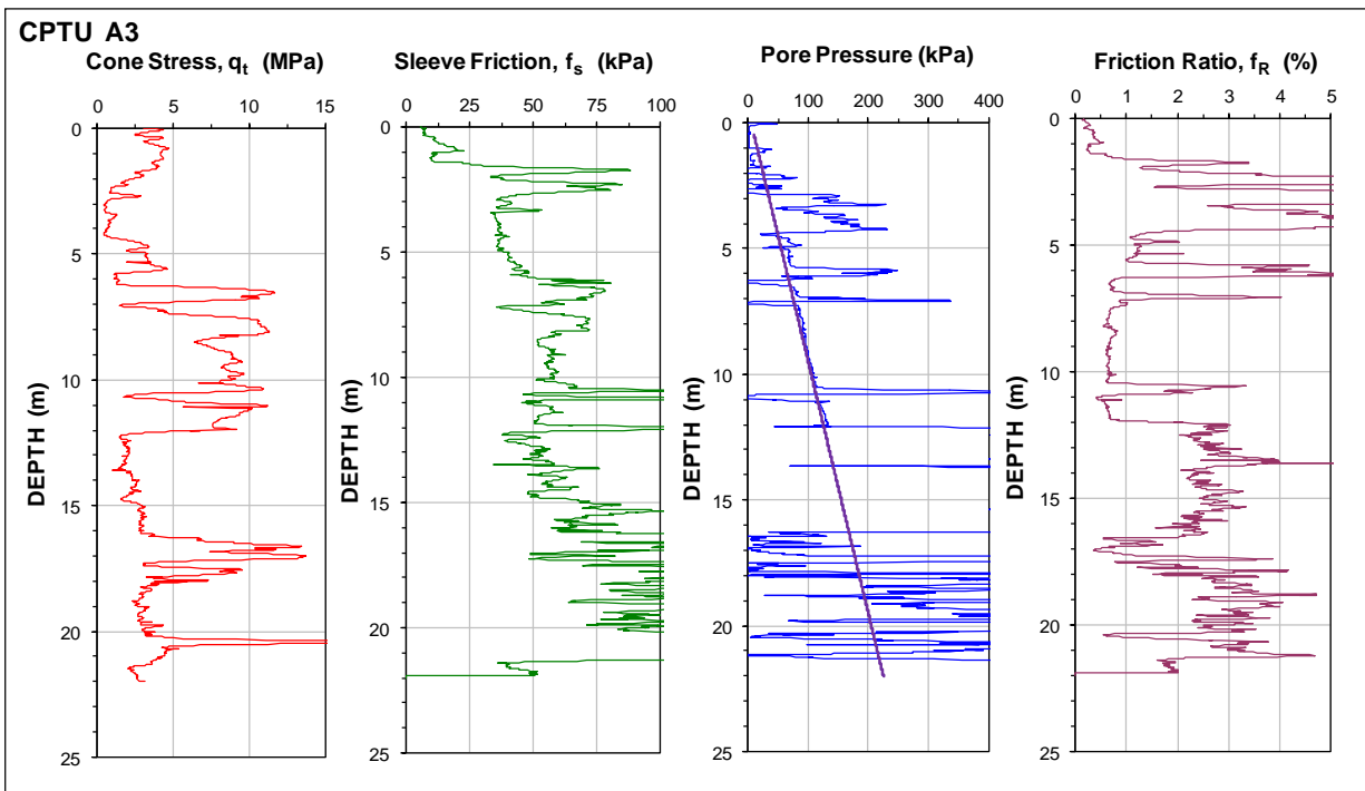
Fig. 19. Results of CPTU A3.
