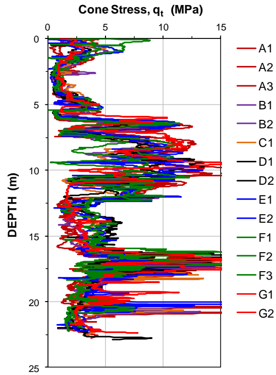
Fig. 16. CPT q_t records from 15 tests.
