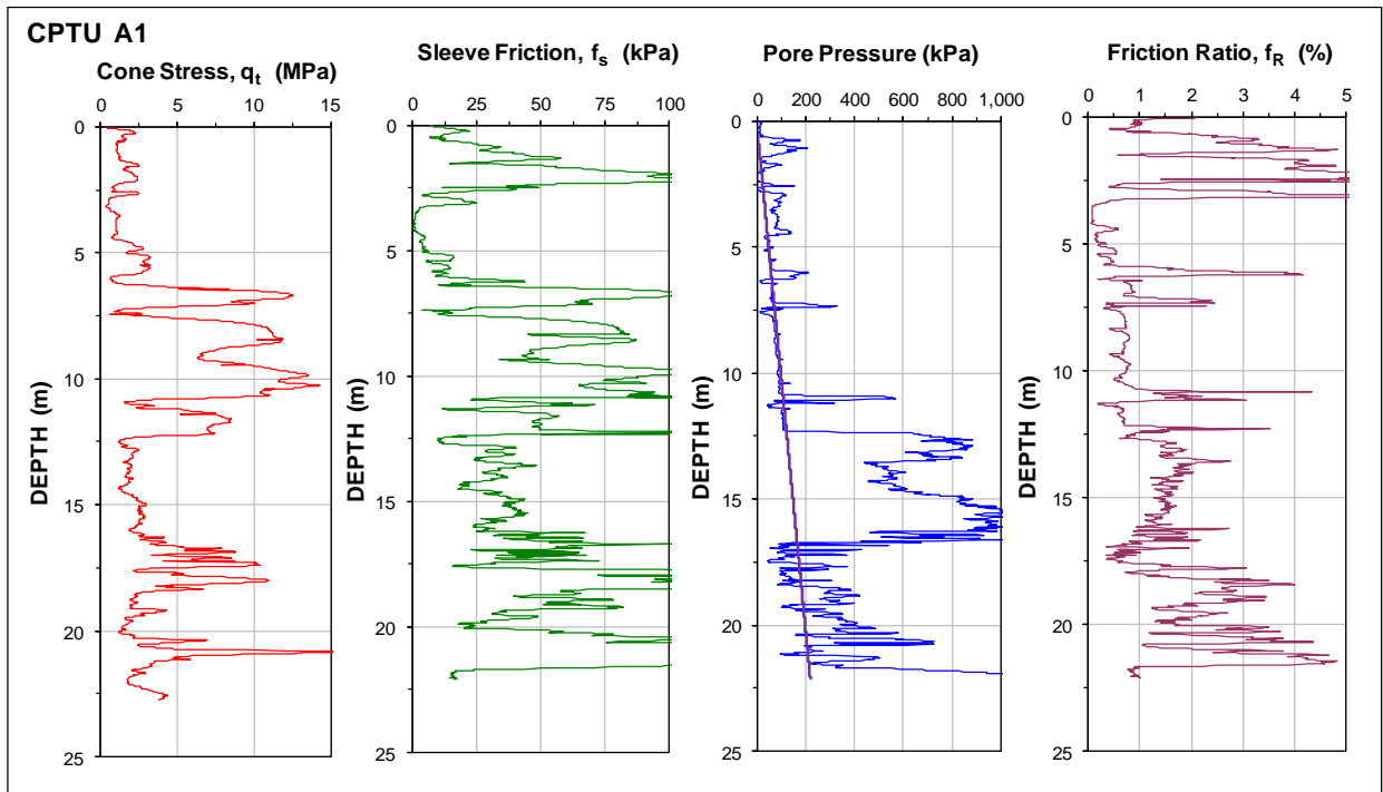
Fig. 17. Results of CPTU A1.
