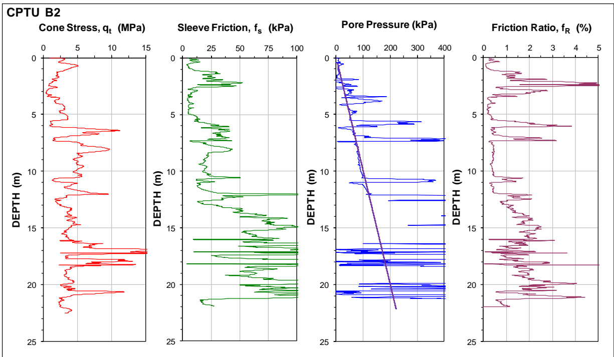
Fig. 21. Results of CPTU B2.
