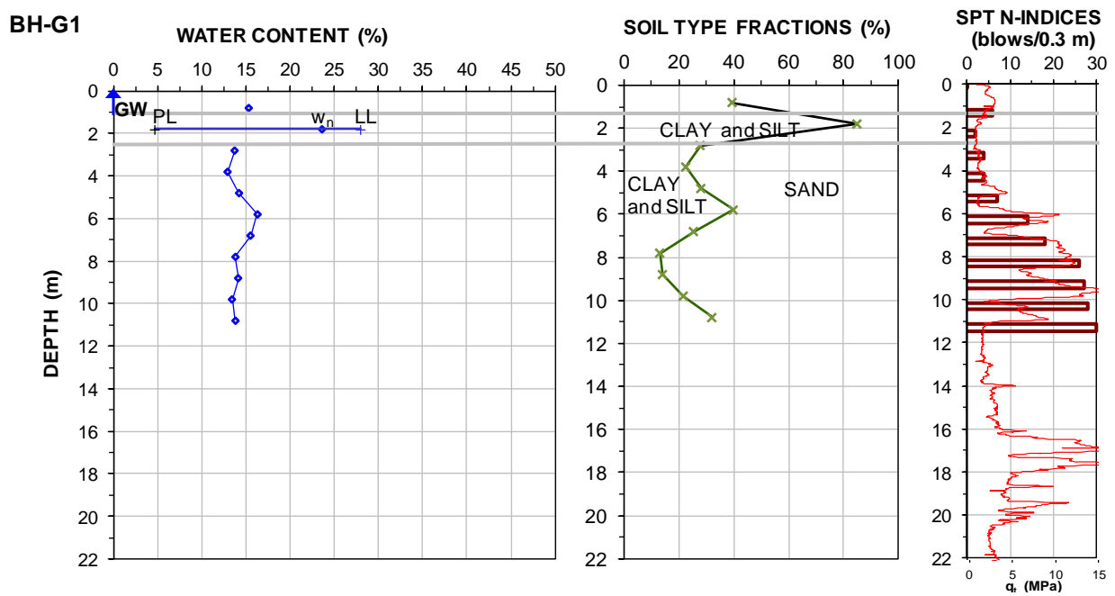
Fig. 15. Borehole data and SPT N-values, BH-G1.
