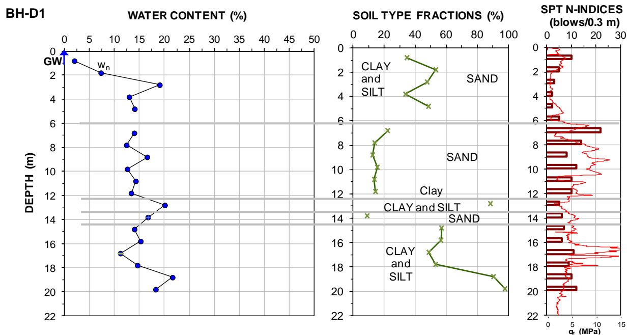
Fig. 11. Borehole data and SPT N-values, BH-D1.
