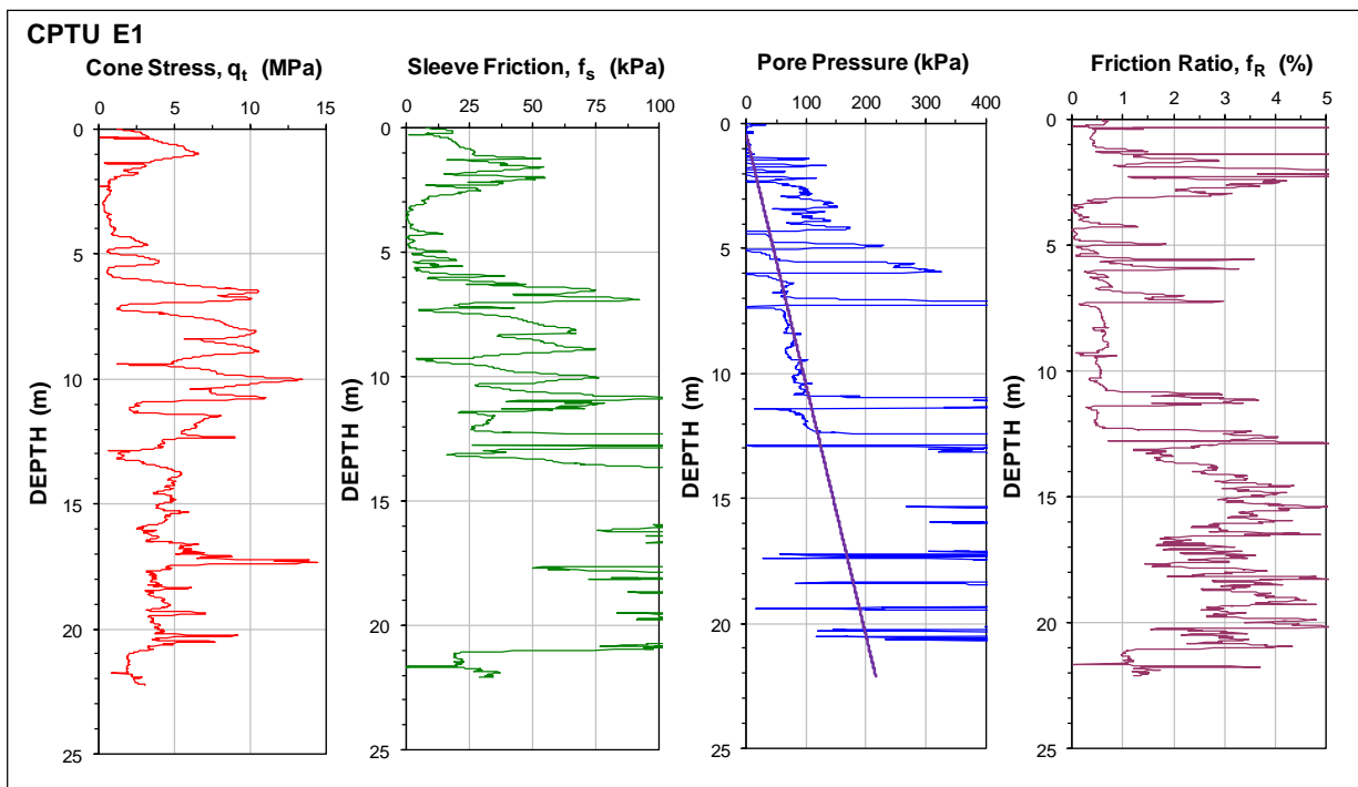
Fig. 25. Results of CPTU E1.
